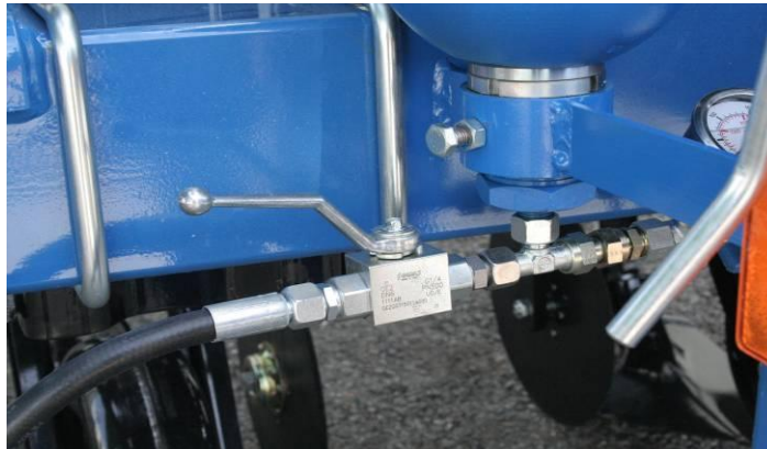
Fig. 13 Hydraulic Pressure Valve in Open Position
