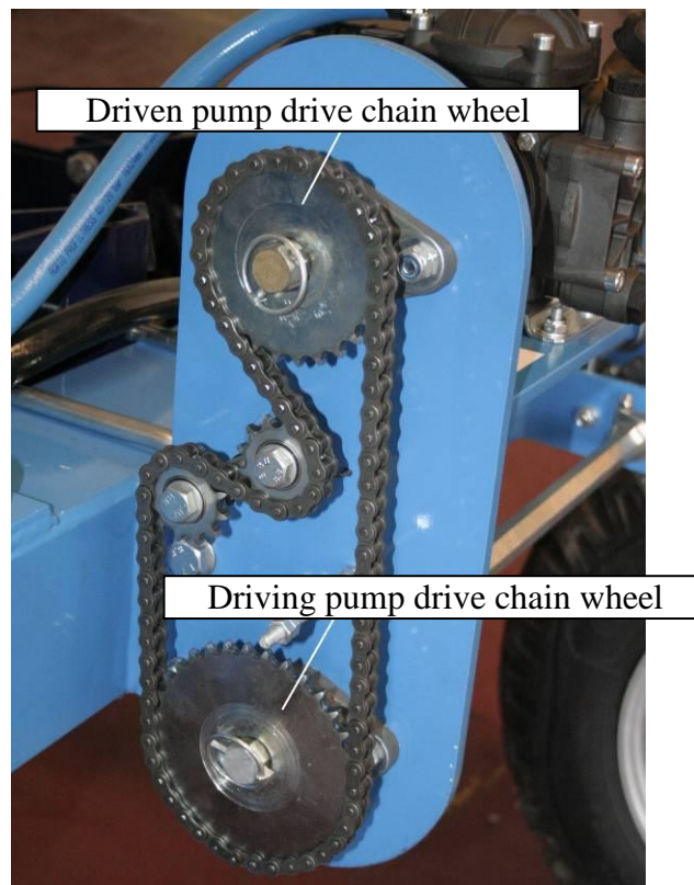
Fig. 5 Chain Pump Gear
