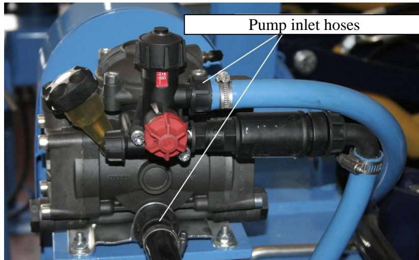
Fig. 14 Attachment of the Pump Inlet Hoses
