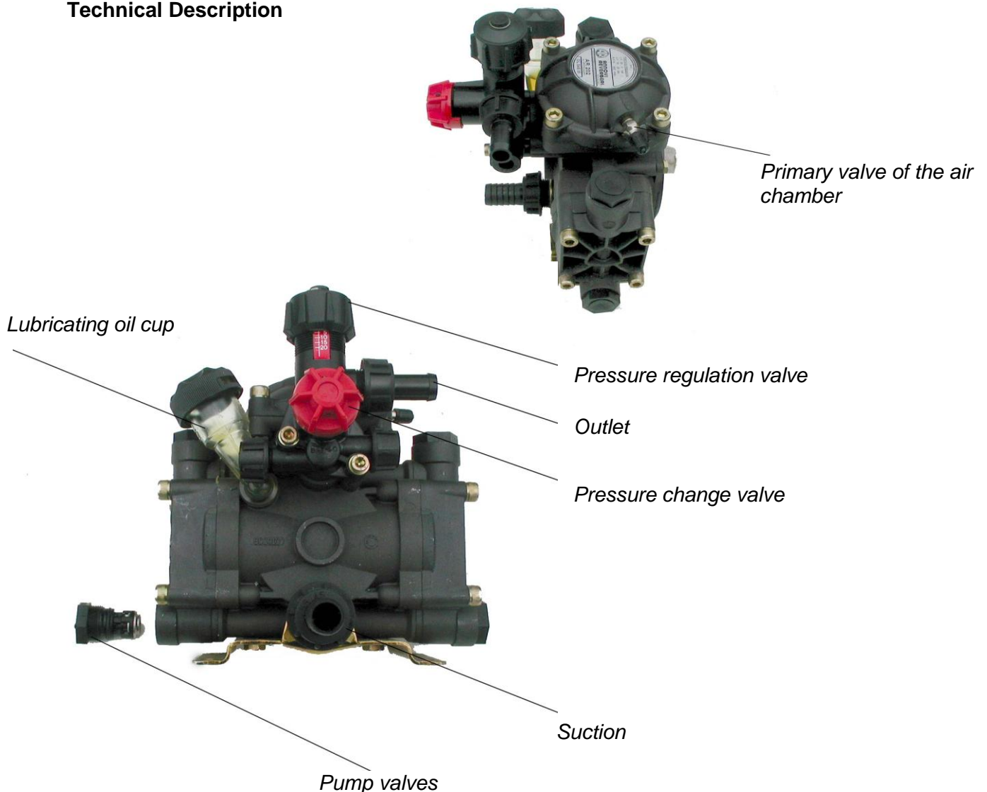
Fig. 2 Pump
