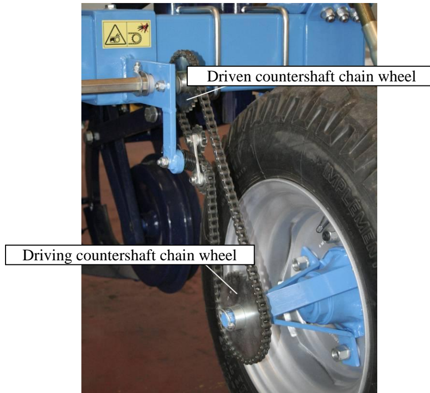
Fig. 4 Chain Countershaft Gear
