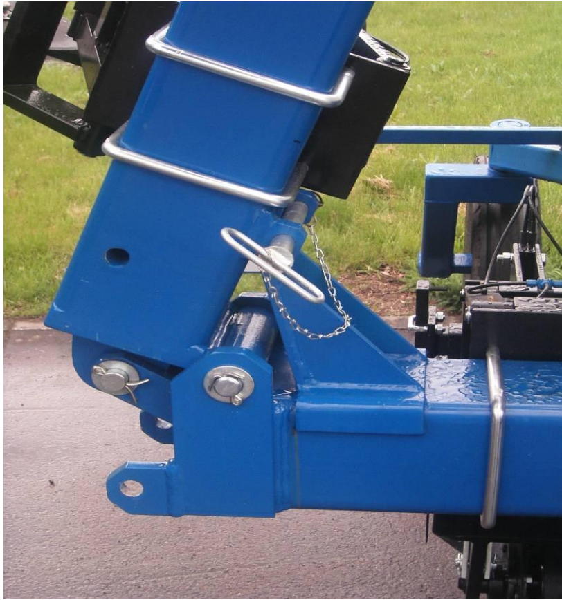
Fig. 9 Arm Secured with Pin in Transport Position
